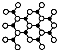
FIG. 6.—Two-dimensional analog of a crystal of AO . (Zachariasen.)
